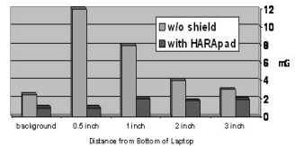
HARApad Magnetic Shielding Performance
